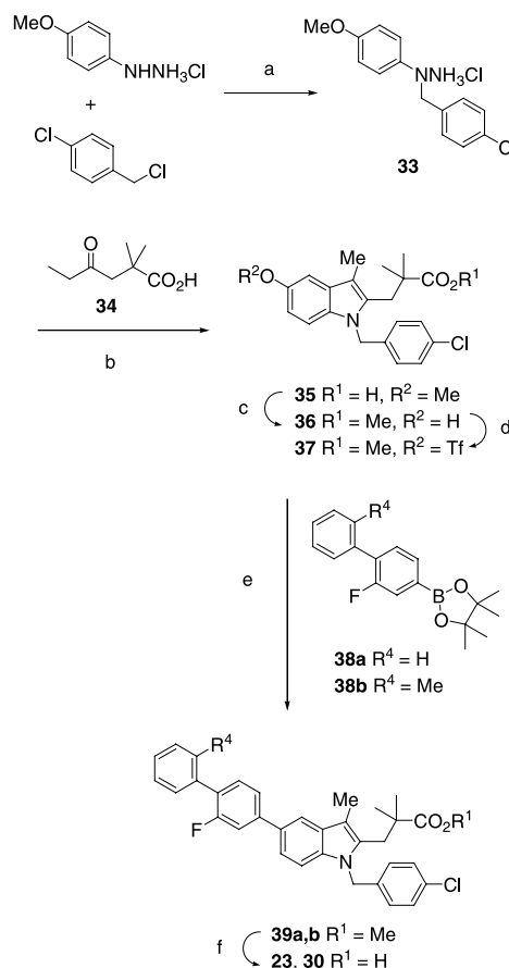
Scheme 1. Reagents and conditions: (a) Et 3 N, PhMe, reflux, 15 h; HCl (52%); (b) t BuOH, reflux, 15 h (54%); (c) BBr 3 , CH 2 Cl 2 , –60 to 0 °C; MeOH (100%); (d) Tf 2 O, Et 3 N, CH 2 Cl 2 , 0 °C (81%); (e) for 38a : PdCl 2 (dppf) (cat.), aq Na 2 CO 3 , DMF, 80 °C, 2 h (40%); for 38b : PdOAc 2 (cat.), PPh 3 (cat.), aq Na 2 CO 3 , DME, reflux, 2 h (99%); (f) LiOH, THF, MeOH, 60 °C, 4 h (82–97%).
